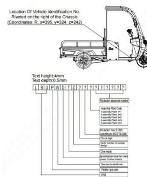
Figure 2-10 VIN code
