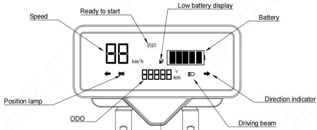
Figure 2-1 Speedometer
